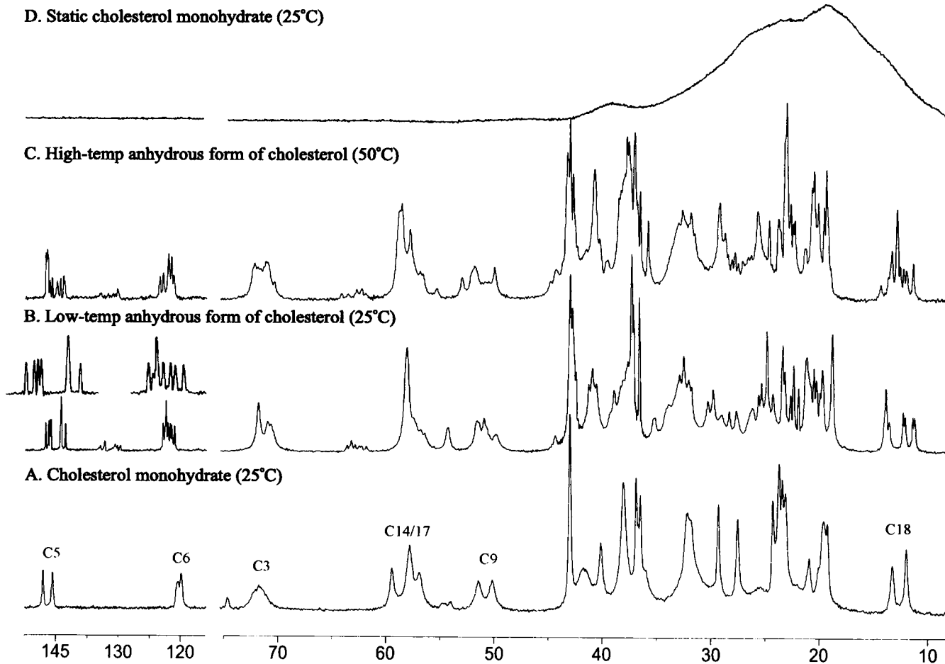
FIGURE 1 The 13 C CPMAS of (A) cholesterol monohydrate, (B) a low-temperature form of anhydrous cholesterol, (C) a high-temperature form of anhydrous cholesterol, and (D) the same sample as in (C) but without spinning. Selected CHOL resonances are identified by the standard numbering system for CHOL. The number of scans was 1000 for each spectrum.
